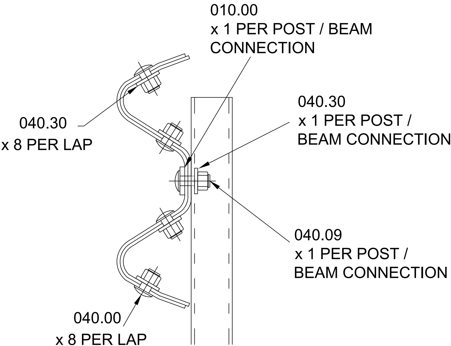
SECTION A-A BEAM LAP AND POST TO BEAM CONNECTION DETAILS
